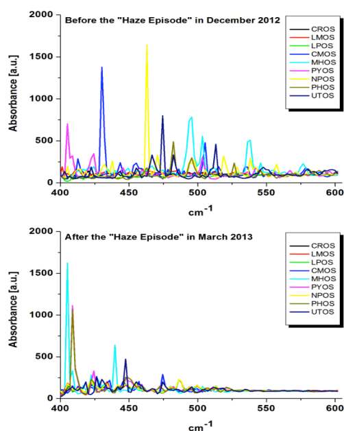
Figure 3. FTIR Spectrum of PM_{2.5} from Wave Number 400 to 600 cm^{-1}
